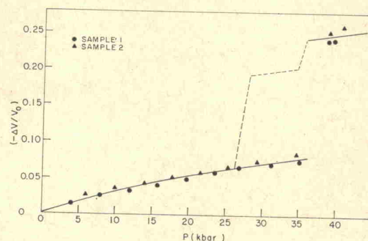
FIG. 6. Compression of CdTe.
